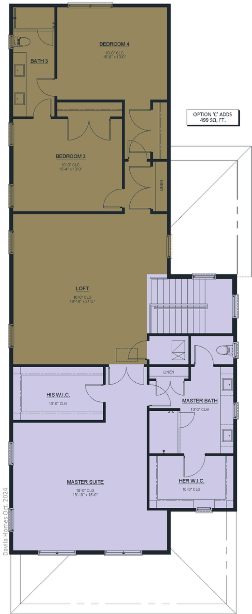
SECOND FLOOR - OPTION C ADDS 499 S.F.
